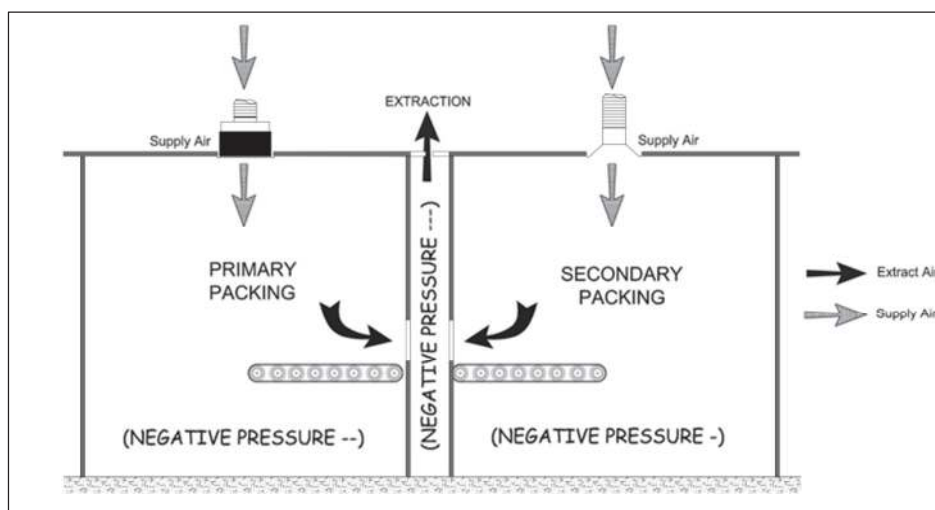
Figure Typical airflow pattern for contaminant
